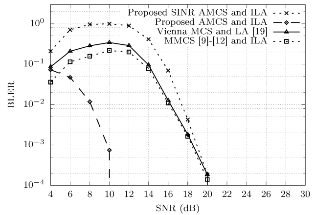
Fig. 7. Block error rate versus SNR for 50 users.
