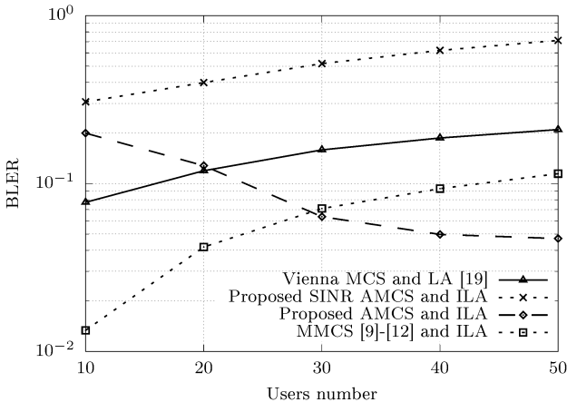
Fig. 6. Block error rate with SNR = 6 dB.
